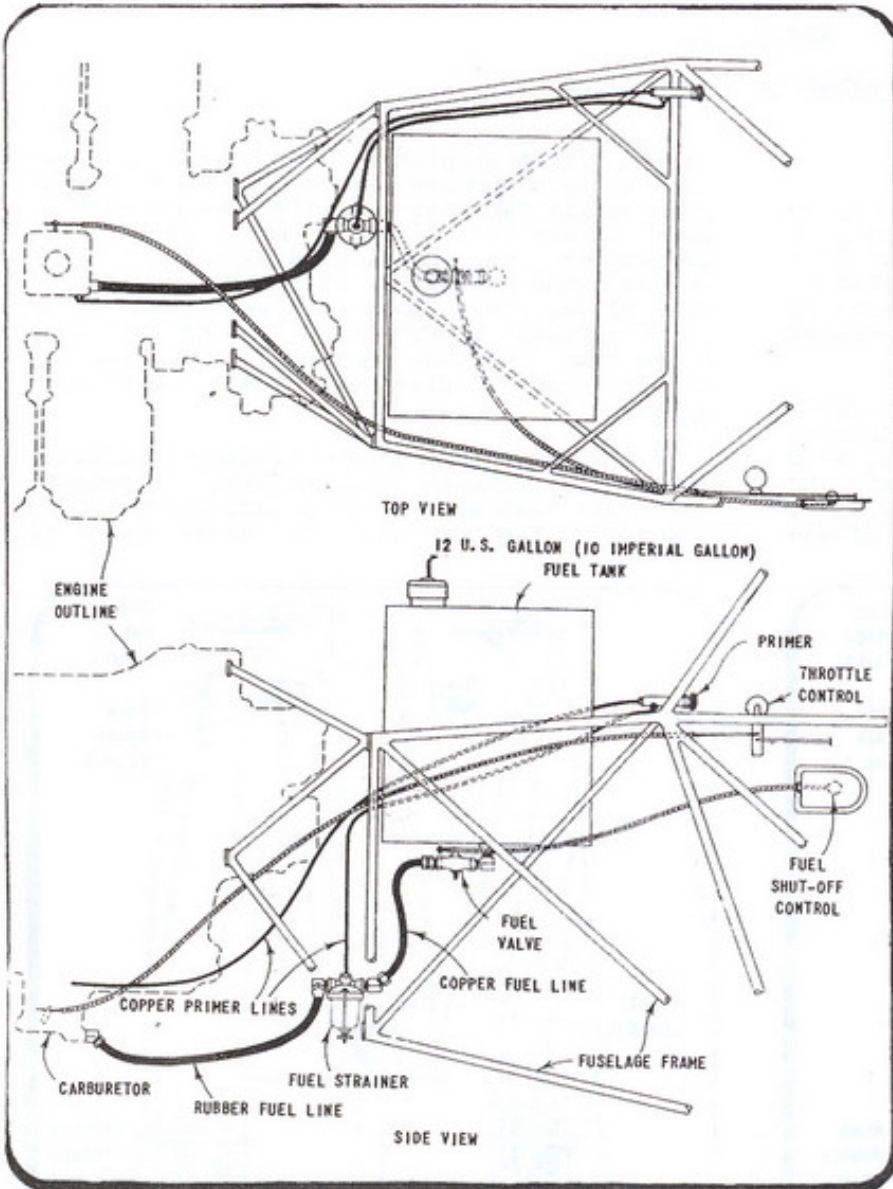
Figure 18 - Fuel System in the Models L-4A and L-4B
