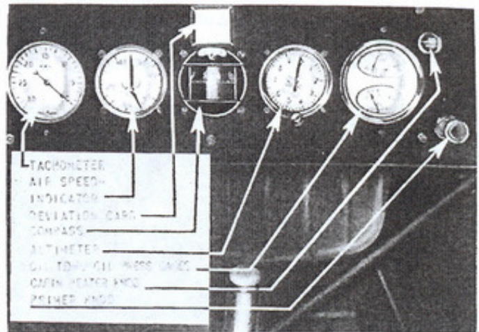
Figure 9 - Instrument Panel on the Model L-4B
